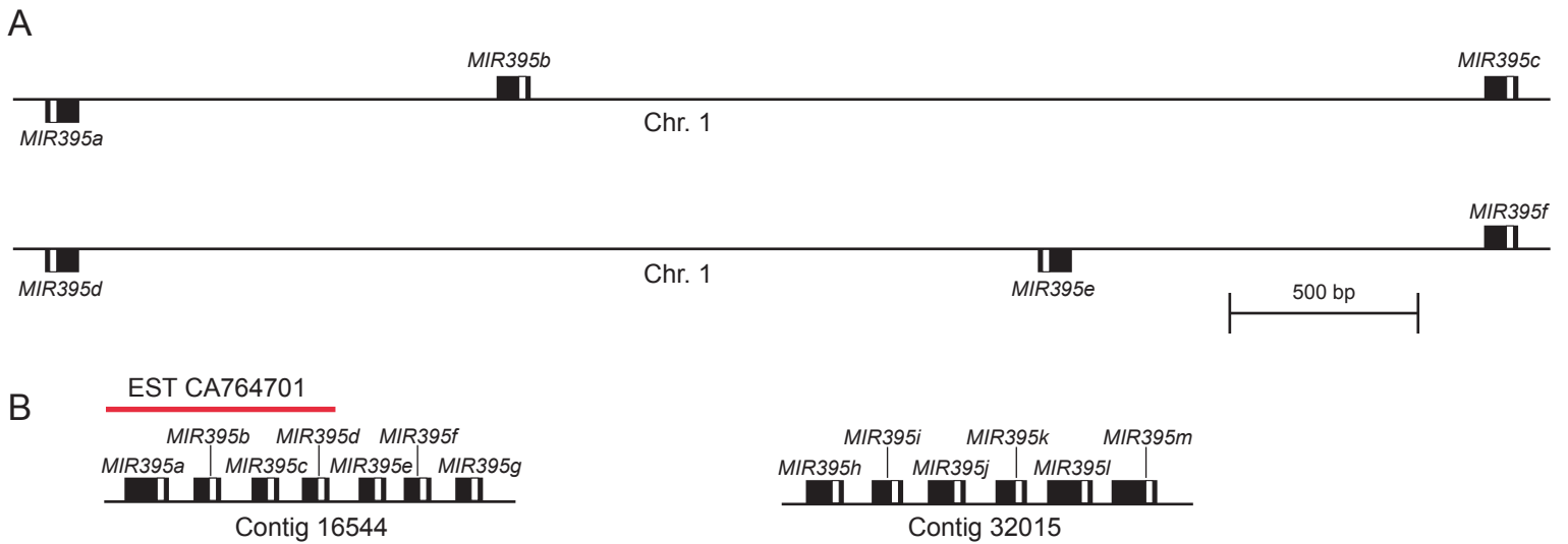
Figure S1. MIR395 clusters in Arabidopsis and Oryza
