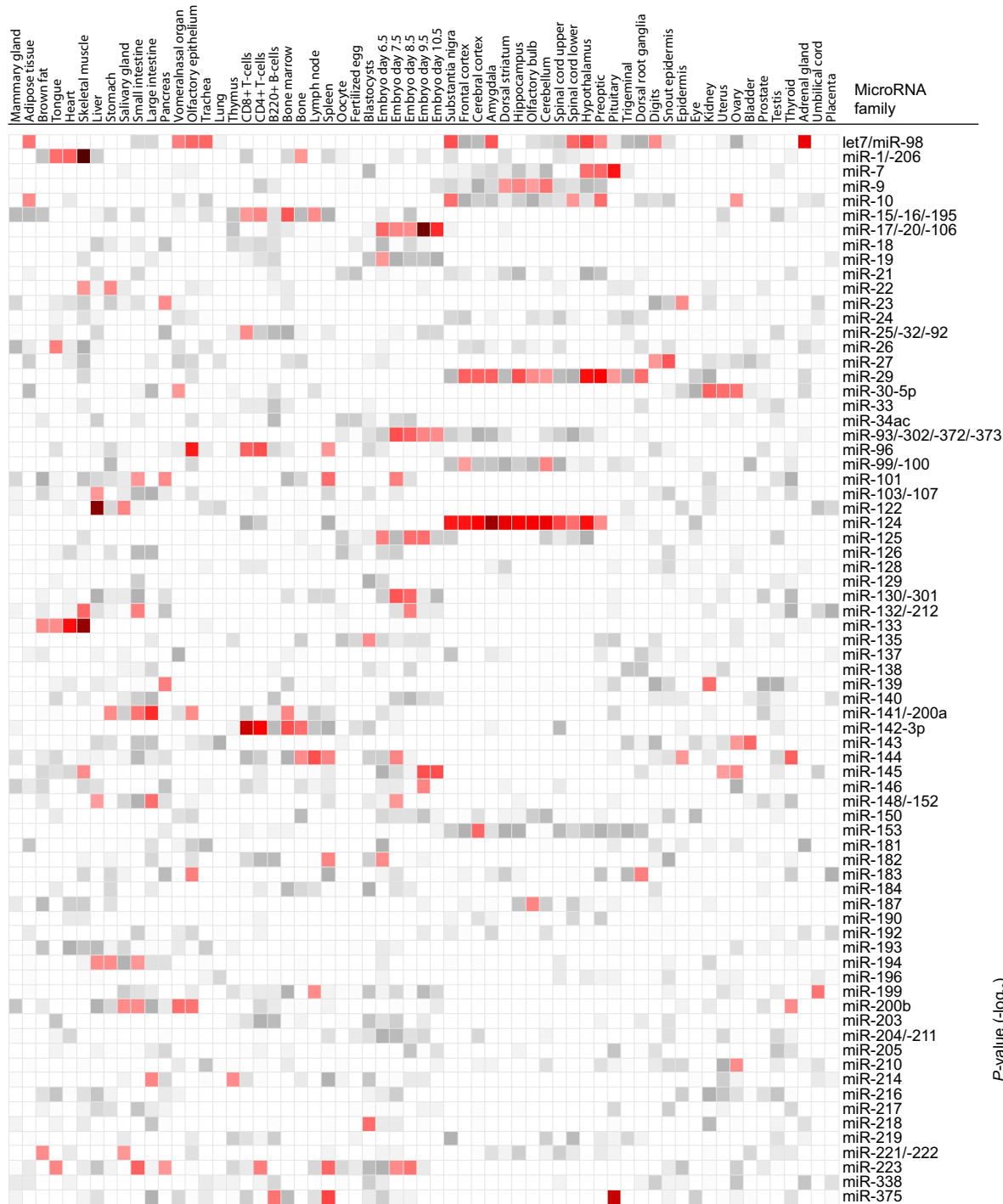
Supplemental fig. S7. Complete map showing KS-test P values for each tissue-miRNA pair (61 tissues, 73 miRNAs) like that shown in Figure 4B. Darker areas denote increasingly significant values (Table S2), as indicated in color key.
